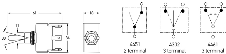
Metal Shaft Toggle Switches
