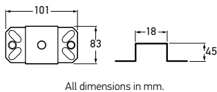
All dimensions in mm.
