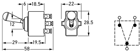
Changeover Switch On-On
