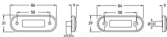
Stainless steel rim version
