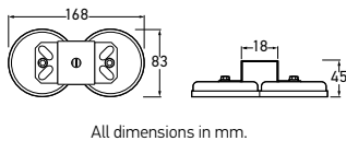
All dimensions in mm.
