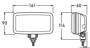
All dimensions in mm.
